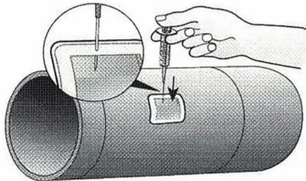
Figure 4 — Water being injected into the compartment in the patch (carefully following the procedure described in 6.3.4 and 6.3.5 )
